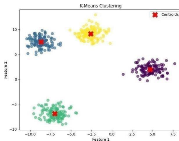
Fig 5.2.10 Clustering Map
