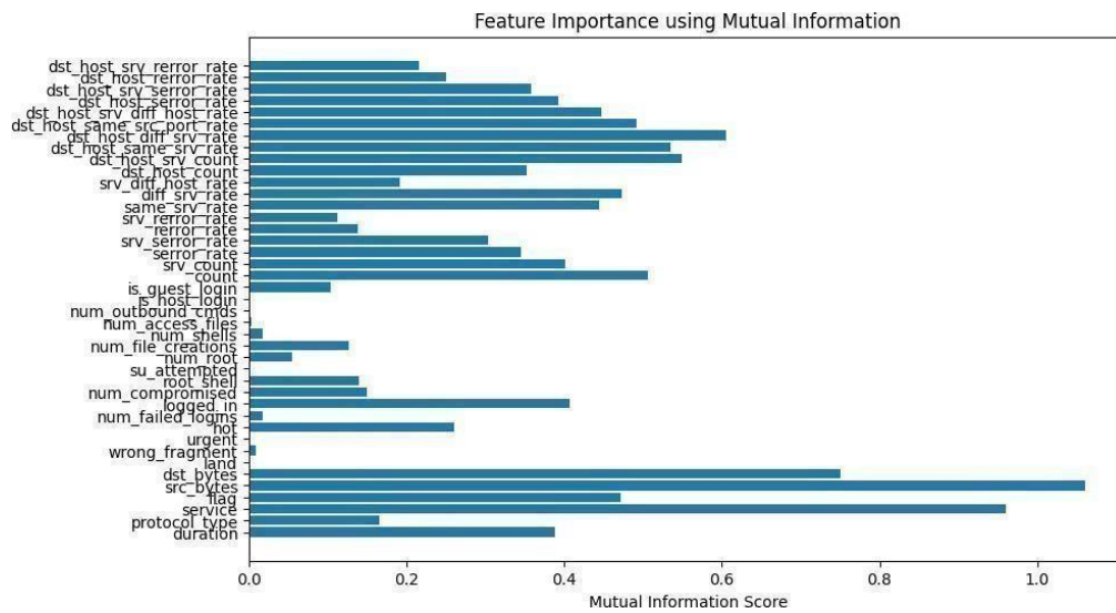
Fig 5.2.9 Feature Importance
